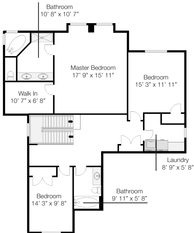
Upper Level 1207 sq. ft.
