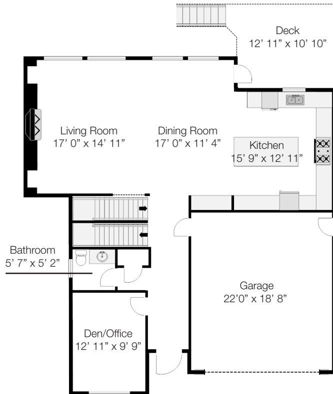
Main Level 1155 sq. ft.
