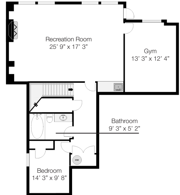
Basement 1098 sq. ft.
